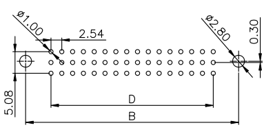
RECOMMEND PCB LAYOUT(FOR FEMALE) TOLERANCE=±0.05mm
