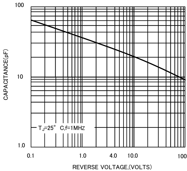
FIG.3-TYPICAL JUNCTION CAPACITANCE
