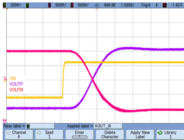
Figure 8-4. Step Response of the AMC1301
