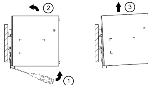
Fig. 3.2 Dismounting
