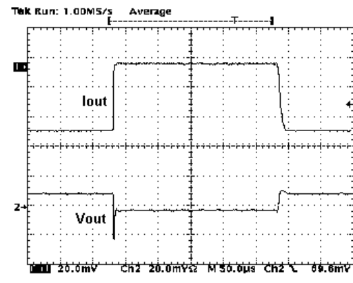
Figure 28 : Load Transient
