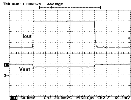
Figure 27 : Load Transient
