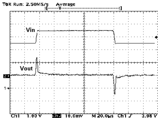
Figure 25 : Line Transient
