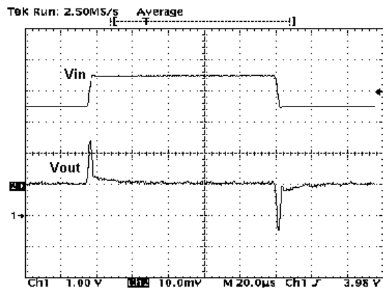
Figure 25 : Line Transient
