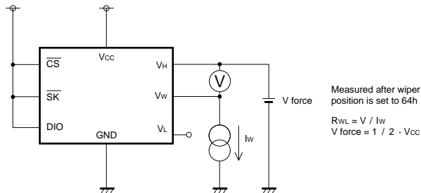
Fig. 9 Wiper resistance measurement circuit on High side
