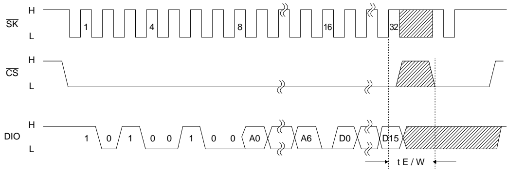
Fig. 15 Data write
