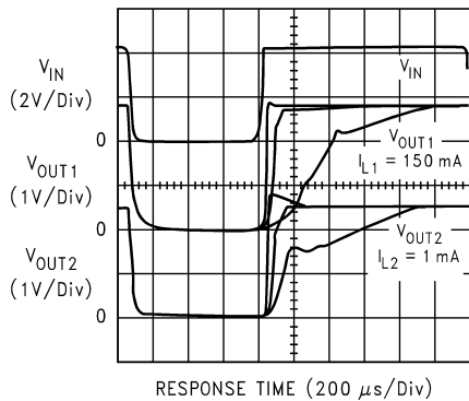
Start-Up Time ( C_{BP} = 0.001, 0.01, 0.1\mu\text{F} )
