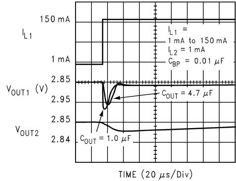
Load Transient & Cross Talk ( V_{IN} = V_{OUT} + 0.2\text{V} )
