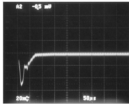
Transient Response for 0–0.5A Load Step
