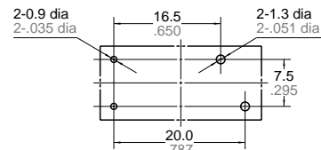
PC board pattern (Copper-side view)
