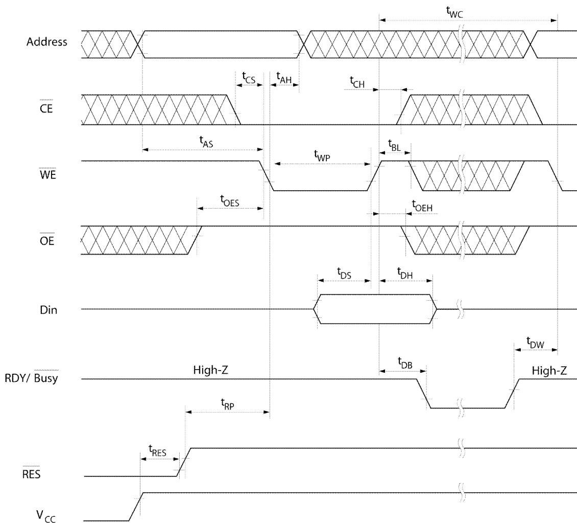
FIGURE 2. BYTE WRITE TIMING WAVEFORM(1) ( \overline{WE} CONTROLLED)
