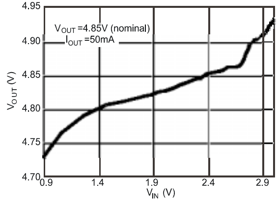
Line Regulation
