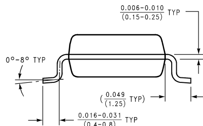
14-Lead Molded Small Outline Package, SOIC EIAJ Package Number M14D
