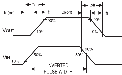
Figure 12. Switching Waveforms
