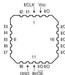
PLCC Top View
